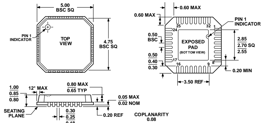
Figure 77. 32-Lead Lead Frame Chip Scale Package [LFCSP_VQ] 5 mm x 5 mm Body, Very Thin Quad Lead (CP-32-8)
